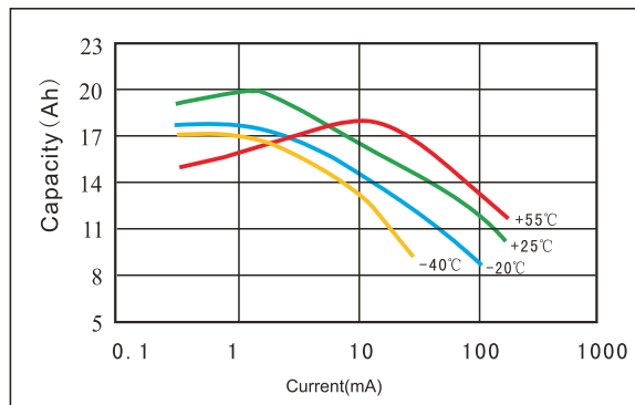
Capacity vs Current curve(cut off with 2.0V)
